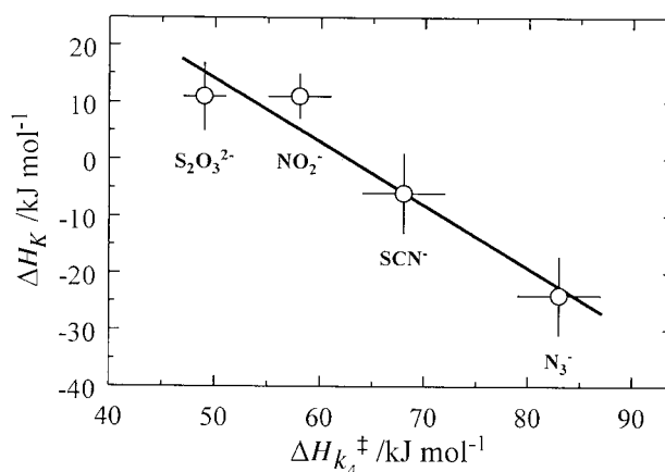
Fig. 4 Inverse correlation of the enthalpy change, \Delta H_K , for formation of the precursor complex [equation (1)] and the enthalpy of activation, \Delta H^\ddagger_{k_i} , for the ligand interchange reaction [equation (2)]. Data from ref. 17
