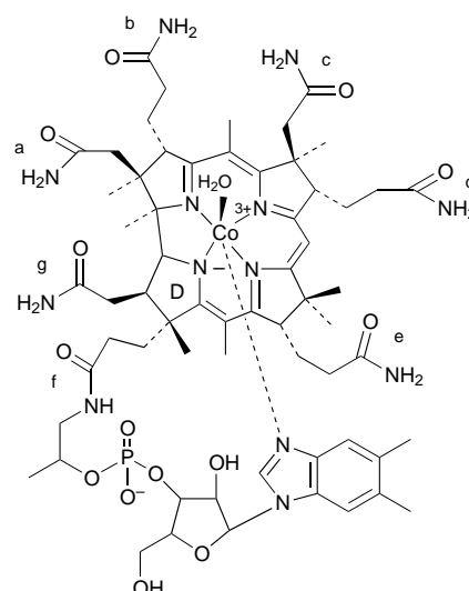
Fig. 1 Aquacobalamin (vitamin B 12a ), in which Co III is co-ordinated in the equatorial plane by corrin. The axial ligand on the lower ( \alpha ) face is 5,6-dimethylbenzimidazole (dmbzim), and that on the upper ( \beta ) face is H 2 O
