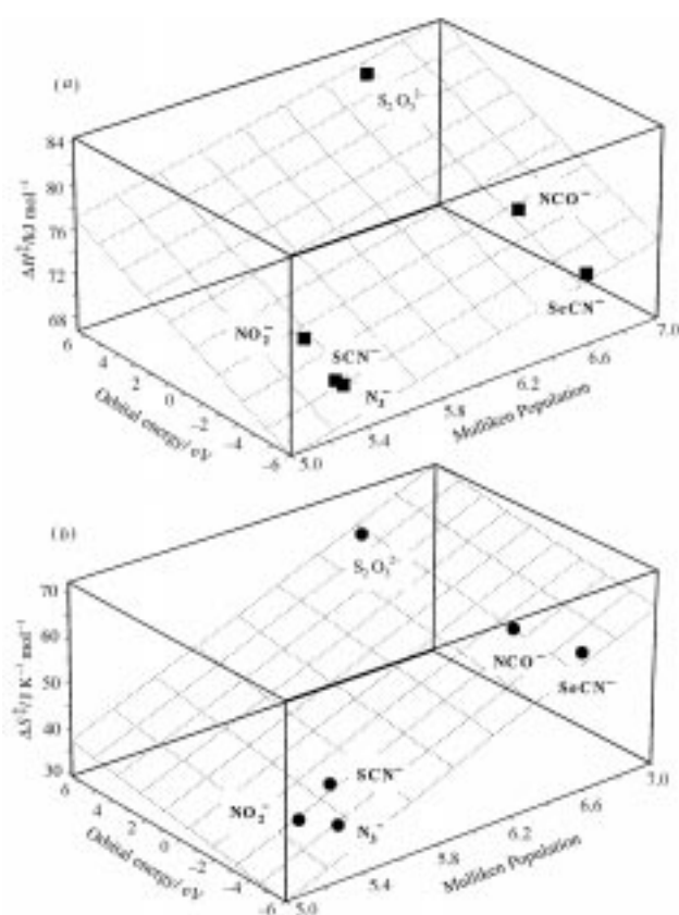
Fig. 5 Correlations between (a) \Delta H^\ddagger_{k_u} and (b) \Delta S^\ddagger_{k_u} and the Mulliken population on the donor atom and the energy of the highest occupied molecular orbital of the ligand, L, with \sigma symmetry
